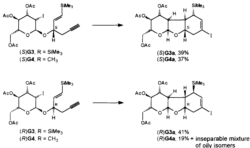
Scheme 8. Rigid, Enantiopure Tricyclic Glycoconjugates via Consecutive 5-exo-dig, 5-exo-dig Cycloisomerization.
