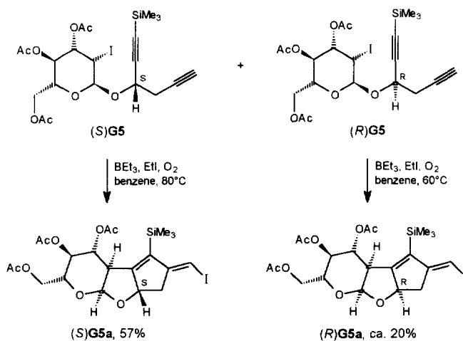
Scheme 8. Rigid, Enantiopure Tricyclic Glycoconjugates via Consecutive 5-exo-dig, 5-exo-dig Cycloisomerization.
