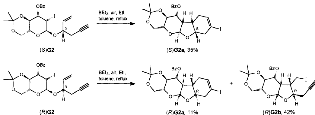
Scheme 6. Remote Acetonide Impedes Conformational Flip: ( S ) vs. ( R ) Series.
