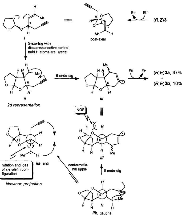
Scheme 4. Configuration and Conformation in the ( R ) Series. Loss of Olefin Configuration, Exemplified for Cyclization of cis -Olefinic Substrate ( R,Z ) 3 .
