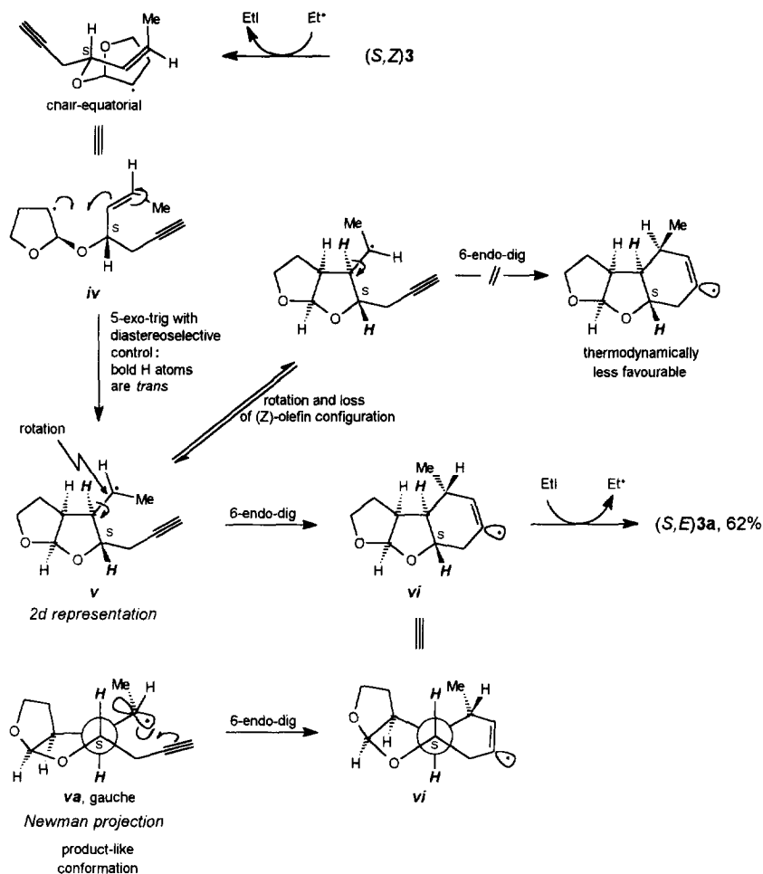
Scheme 5. Configuration and Conformation in the ( S )-Series. Loss of Olefin Configuration, Exemplified for Cyclization of cis -Olefinic Substrate ( S,Z )3.
